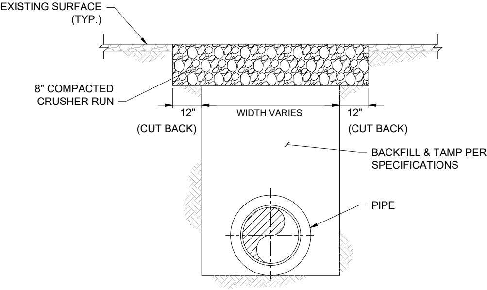
TYPE "B" CUT REPAIR DETAIL DIRT OR GRAVEL RDS (DRIVEWAYS, A-30)
