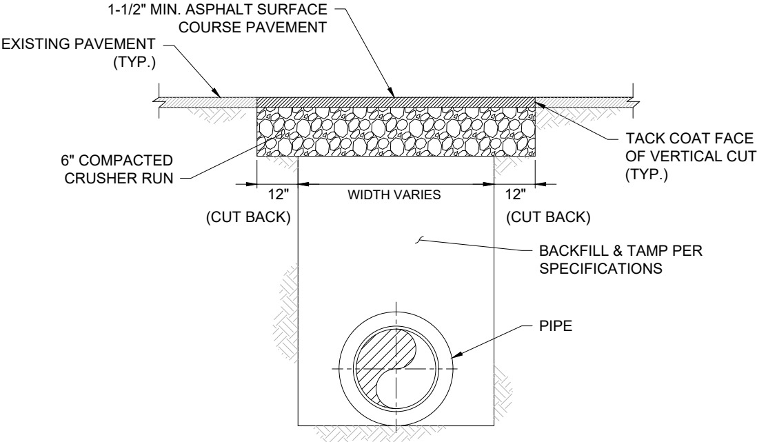
TYPE "A" CUT REPAIR DETAIL T&G OR ASPHALT RDS (DRIVEWAYS, A-30)
