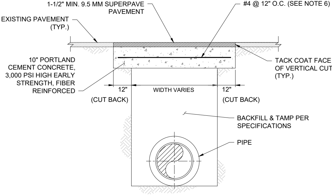
TYPE "C" CUT REPAIR DETAIL GEORGIA DOT AND FULTON CO.
