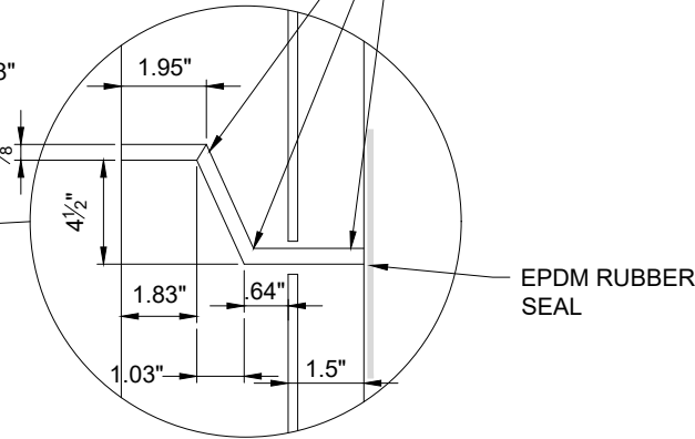
TYPICAL JOINT NTS
