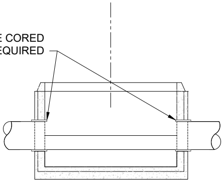
SECTION "A-A" THRU ONE PIECE BASE UNIT NTS
