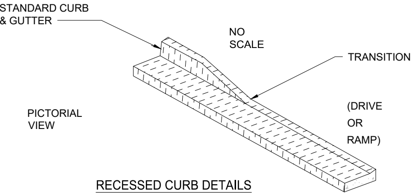
RECESSED CURB DETAILS TYPICAL USE: AT DRIVEWAYS OR CURB CUT RAMPS
