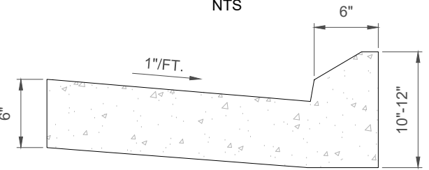
TYPE 2 CONCRETE CURB & GUTTER MAJOR & MINOR RESIDENTIAL SIDE STREETS ONLY
