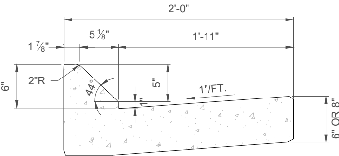
TYPE 3 MOUNTABLE CURB & GUTTER
