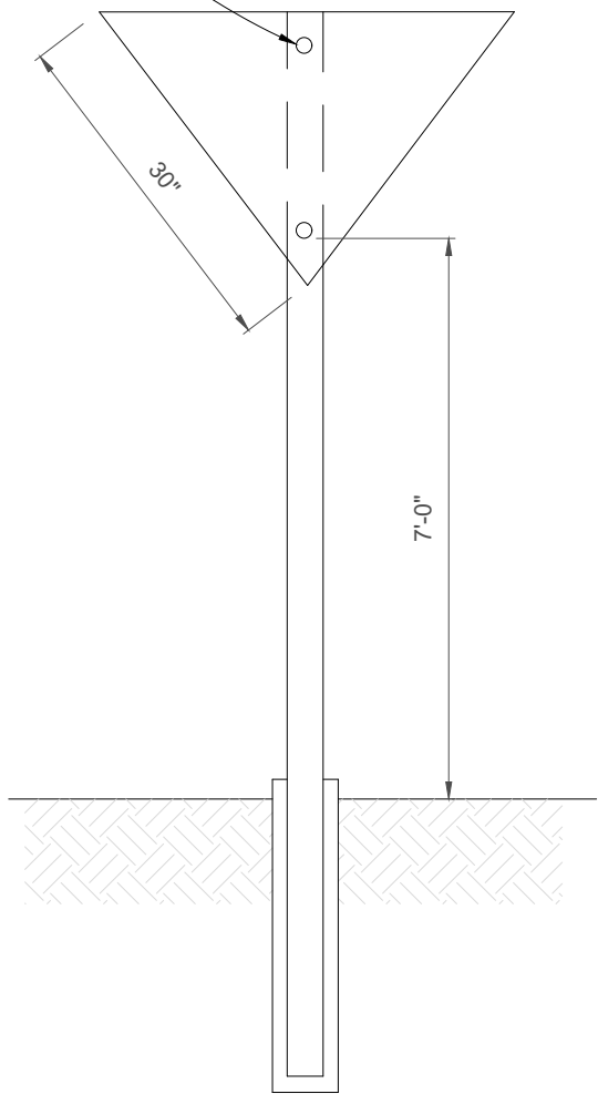
YIELD SIGN DETAILS NTS
