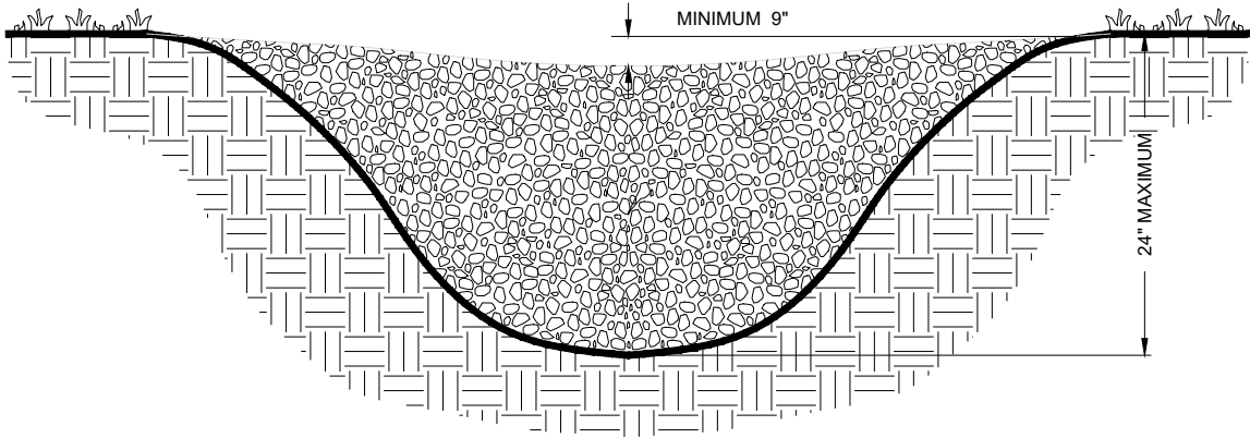
CROSS SECTION
