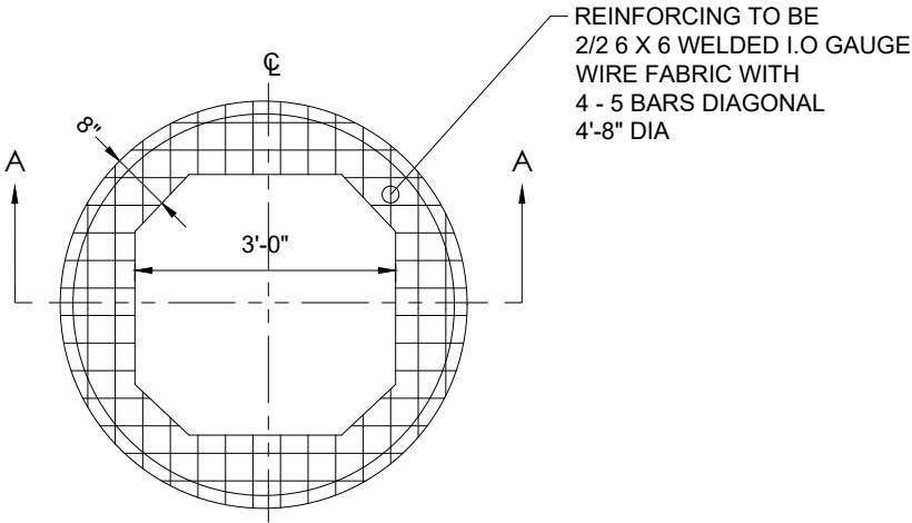
ROUND TO SQUARE ADAPTER
