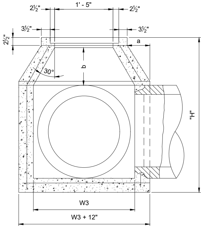
SECTION B-B
