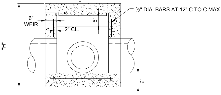
TYPE B SEE SHEET NO. 511 FOR DIMENSIONS
