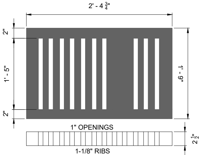
DETAIL OF CAST IRON GRATING APPROX. WT. 200 LB.
