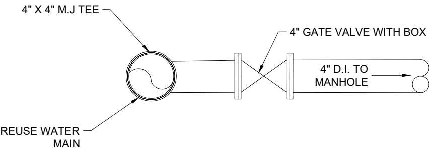
CULC-DE-SAC REUSE TAP AND VALVE DETAIL
