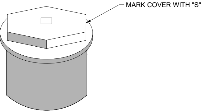
USF 7635 SEWER VALVE BOX AND COVER N.T.S.
