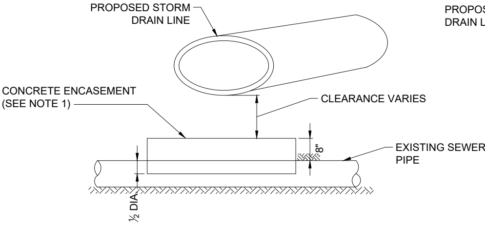
SECTION C - C
