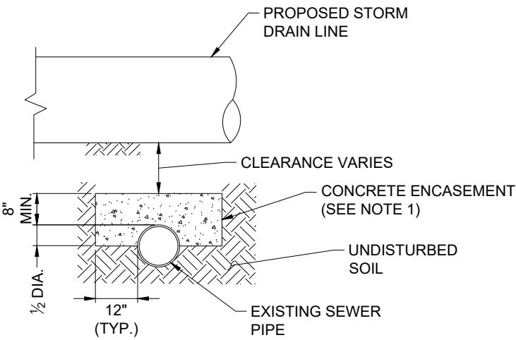
SECTION B - B WITH CONCRETE ENCASEMENT
