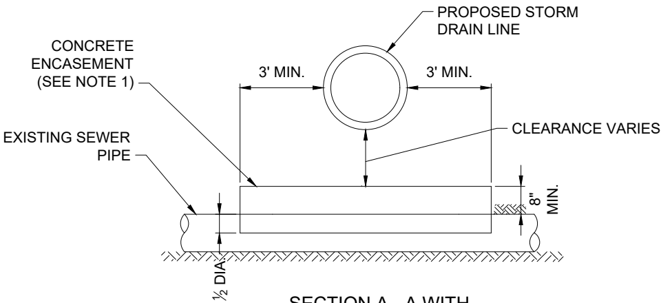
SECTION A - A WITH CONCRETE ENCASEMENT
