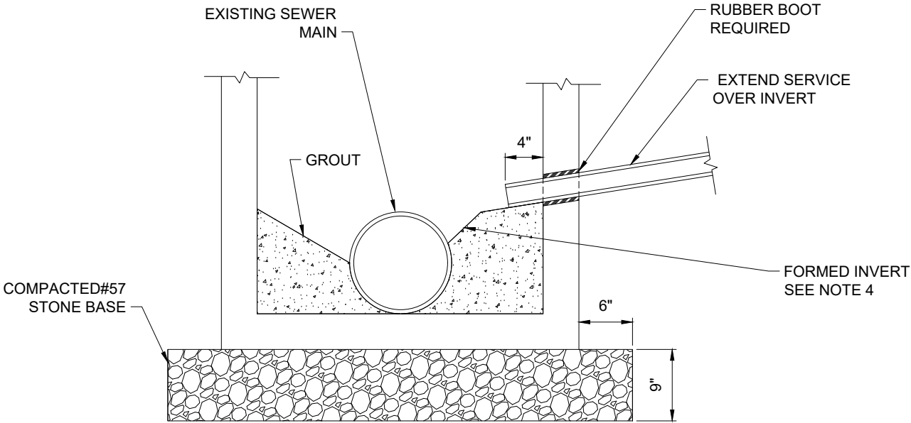
CROSS SECTION AT EXISTING SEWER MAIN (B-B)
