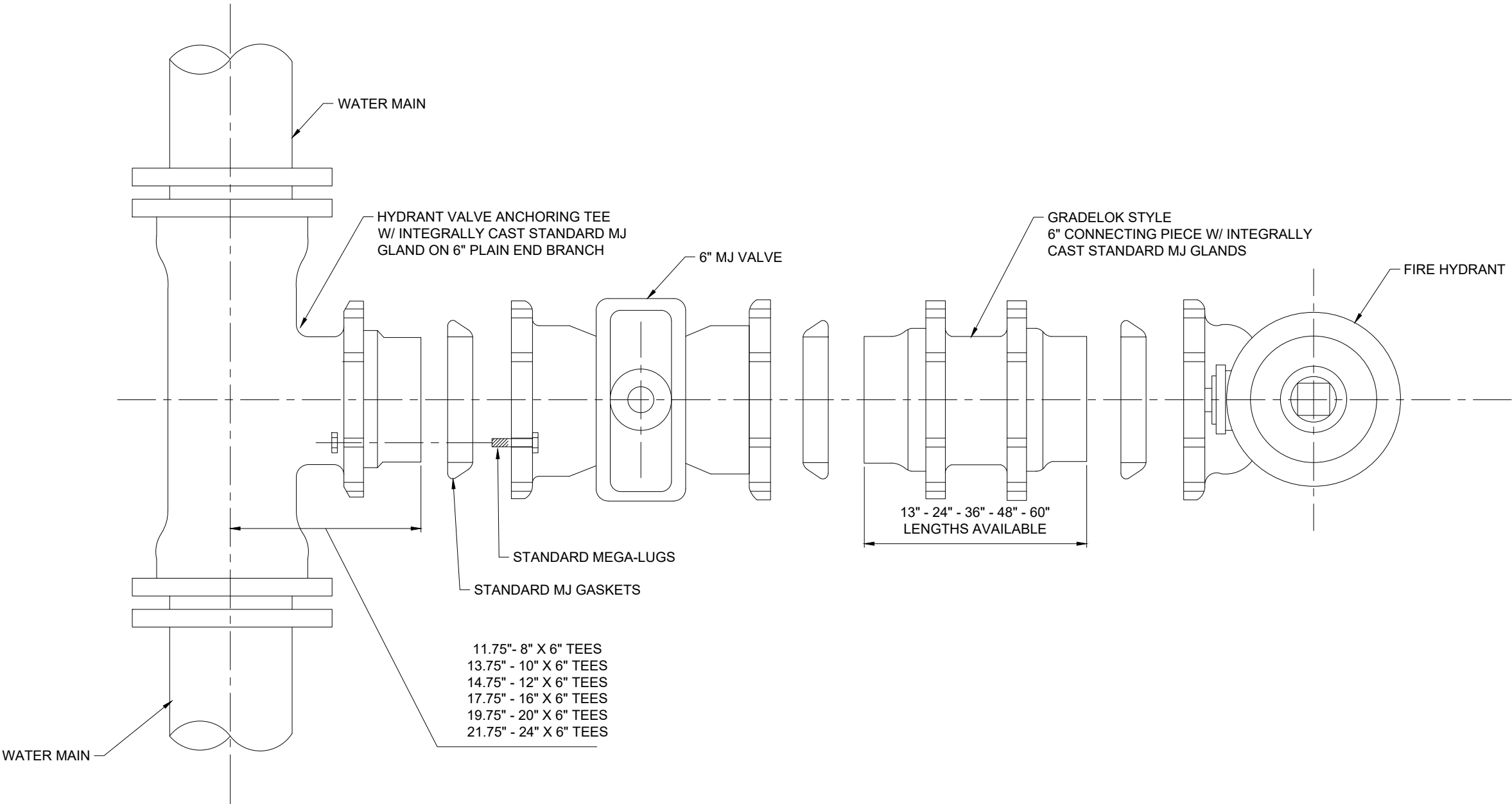
HYDRANT ASSEMBLY DETAIL NTS
