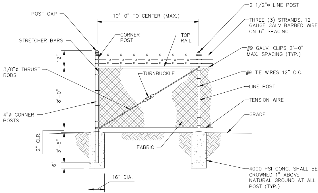
FENCING – CORNER DETAIL N.T.S.
