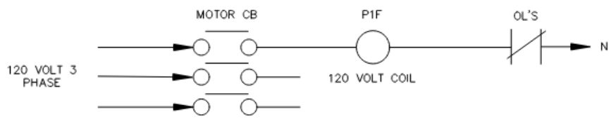
TYPICAL FOR 240V 3 PHASE POWER
