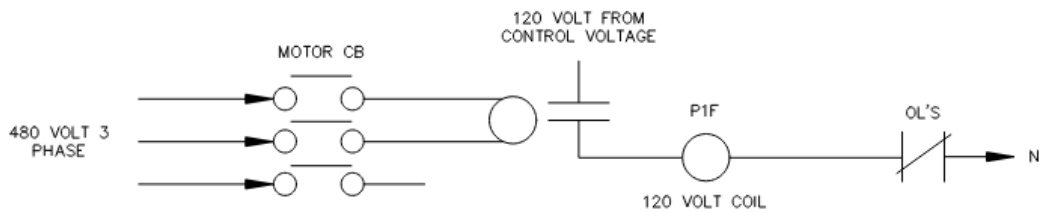
TYPICAL FOR 480V 3 PHASE POWER (PREFERRED)
