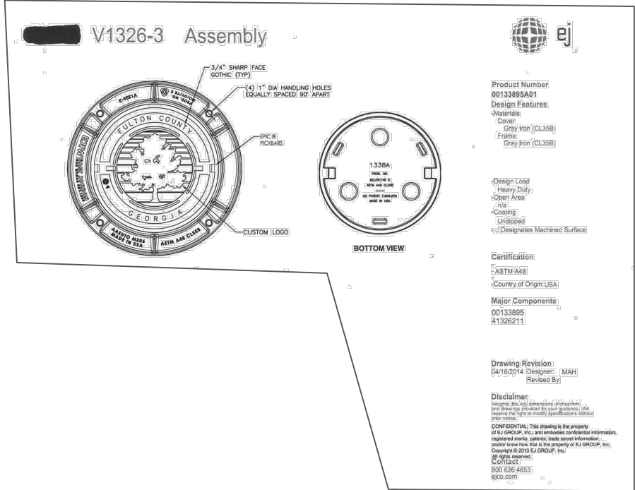
MANHOLE COVER IN A PAVED AREA NOT TO SCALE
