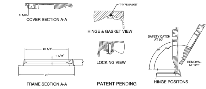
MANHOLE COVER IN A LANDSCAPED OR NATURAL AREA NOT TO SCALE
